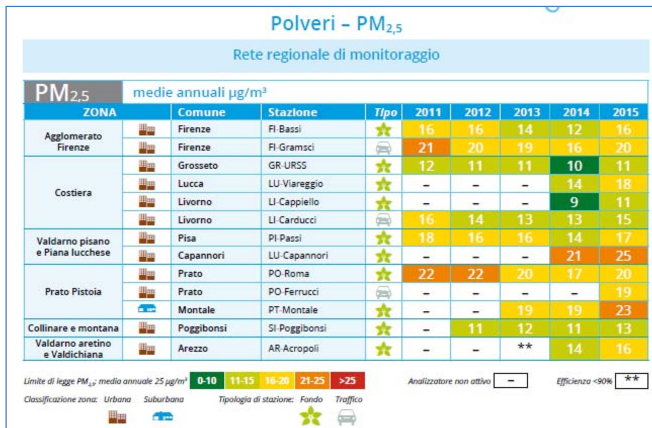
Fig. 3.18 – livelli PM2.5 – medie annuali
