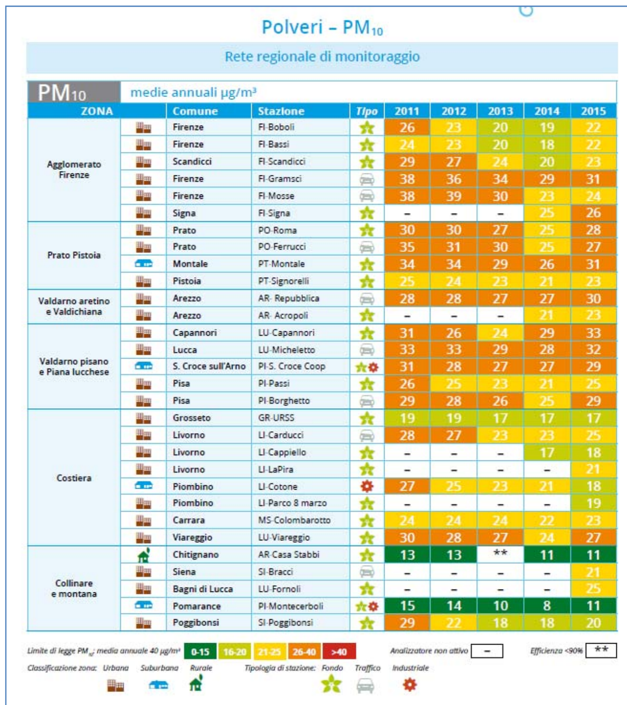
Fig. 3.16 – livelli PM10 – medie annuali
